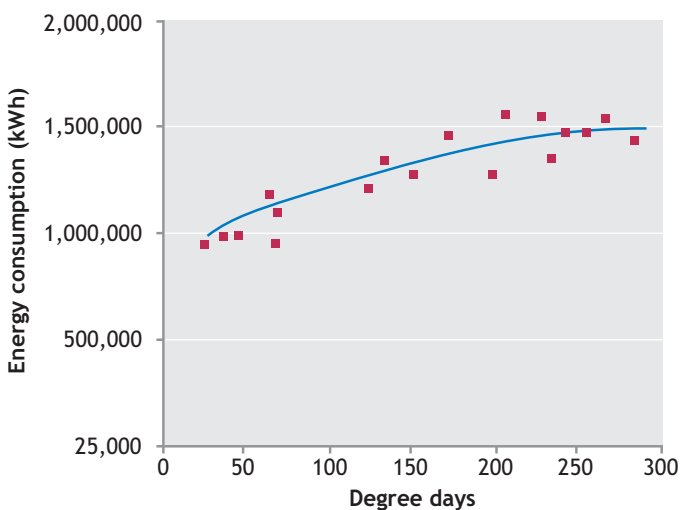
Figure 4c Curve becomes less steep
