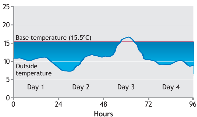
Figure 1 The shaded area is the degree-day value for the period
