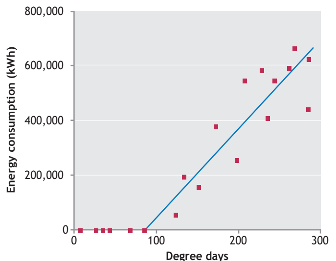
Figure 4b Straight line with intercept on the degree-day axis
