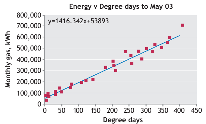
Figure 5 (Figure 4a with equation shown)
