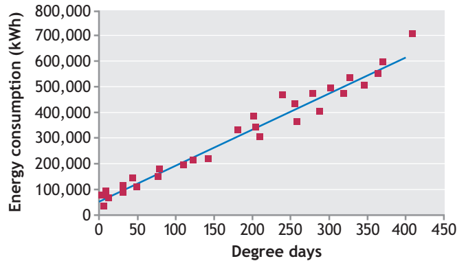
Figure 4a Straight line with a positive intercept on the energy axis and modest scatter
